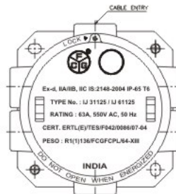
FIG-2 (6 WAY)
