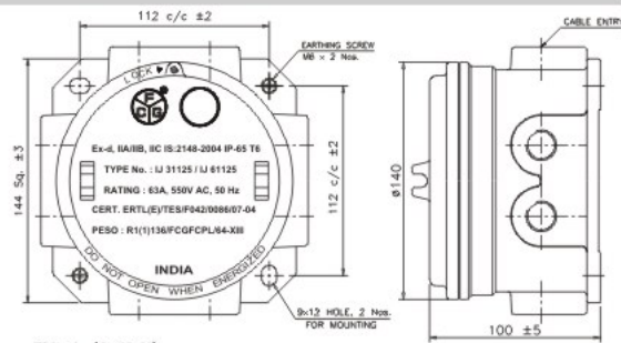
FIG-1 (8 WAY)
