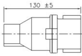
PLUG DETAIL
